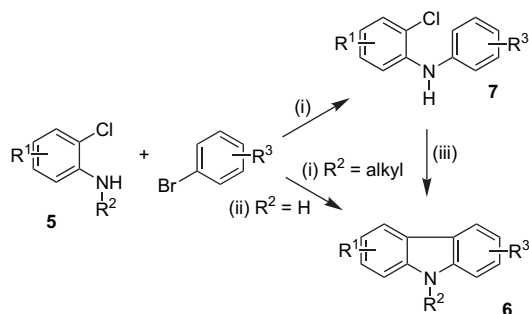
Scheme 7. Pd-PtBu 3 catalysed formation of carbazoles by sequential amination; C–H activation reactions. Conditions: (i) reflux in toluene; (ii) microwave heating in toluene; (iii) reflux in 1,4-dioxane.
