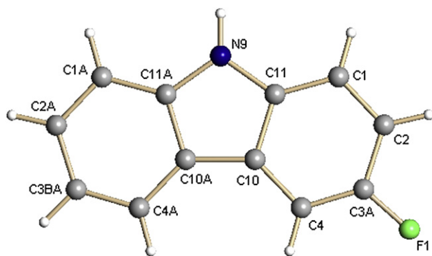
Figure 2. Crystal structure of carbazole 6w , disorder not shown.
