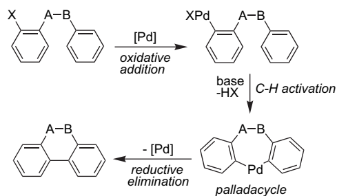
Scheme 4. Generalised reaction pathway for intramolecular direct arylation.
