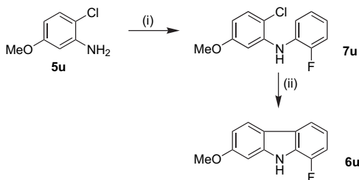
Scheme 8. Conditions: (i) 5u (1 mmol), 2-FC 6 H 4 Br (1 mmol), NaO t Bu (5 mmol), Pd(OAc) 2 (5 mol %), [HP t Bu 3 ][BF 4 ] (7 mol %), toluene, Δ, 18 h. (ii) 7u (0.5 mmol), Pd complex (5 mol %), ligand (7 mol %), base (2.5 mmol), solvent (3 ml), Δ, 18 h—see Table 2 for catalysts, solvents and bases.
