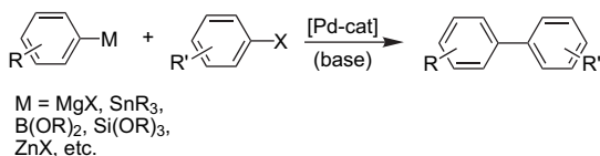
Scheme 1. Cross-coupling reactions.
