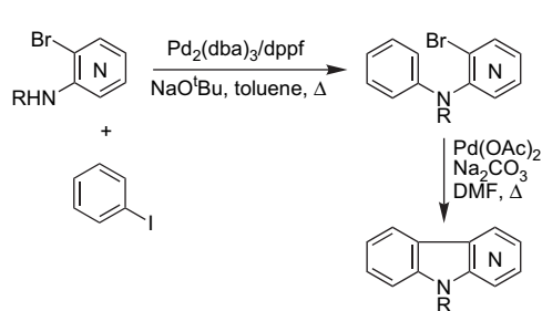
Scheme 5. Synthesis of carbolines via sequential amination and C–H activation.
