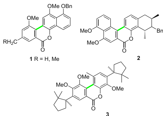
Figure 1. Natural products with pyranone structures formed by C–H activation; the bonds formed during the annulation are highlighted.
